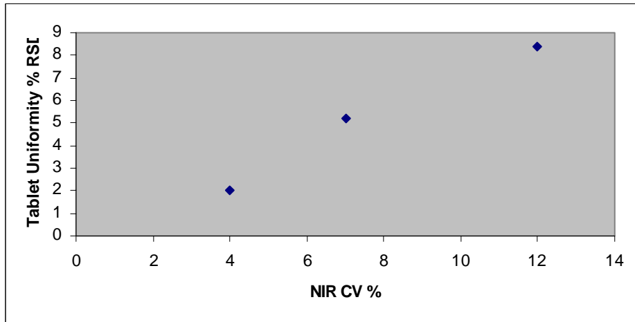
942 Figure 10: Correlation of Blend NIR CV with Tablet Content Uniformity RSD
