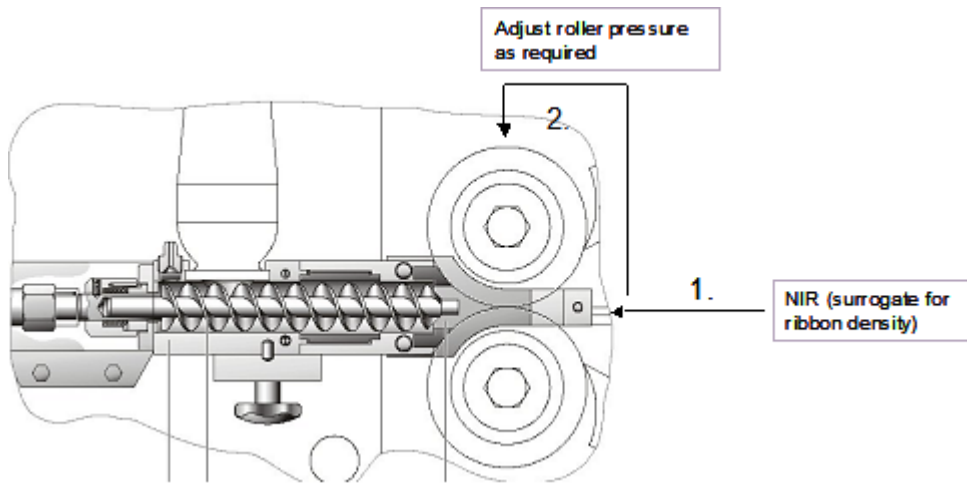
1369 Figure 29: NIR in-process control feedback loop
